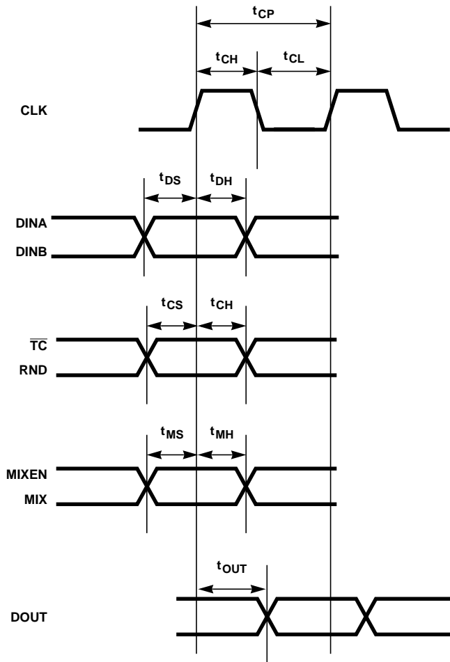
FIGURE 4. SYNCHRONOUS TIMING
